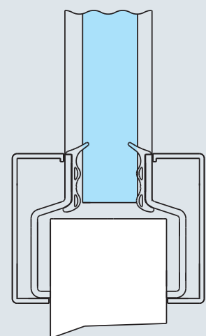
Aluminium-Abdeckprofil
